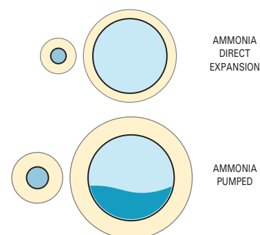
Ammonia pipe comparison
