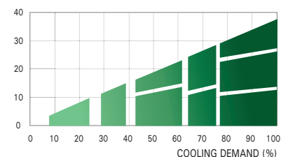
Neutral band suction pressure
