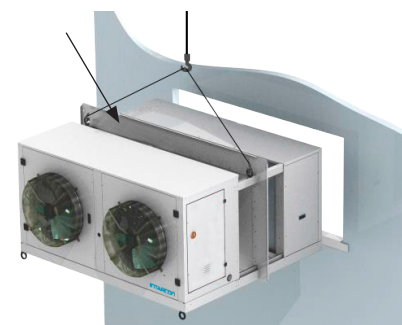
MOUNTING FRAME
